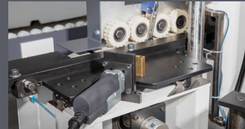
Servo Kontrollü Ön Siper Servo Controlled Entrance Fence
